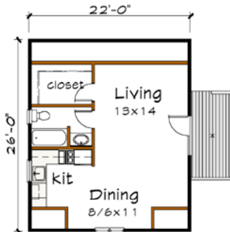
Floor 2 plan
